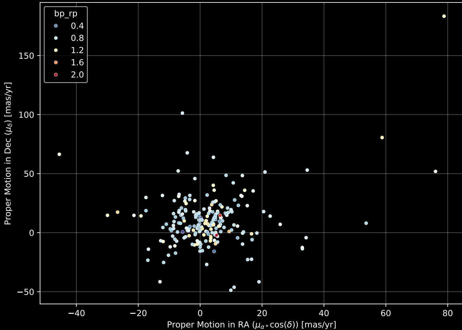
GALAH DR4 Field: [7185] Proper Motion Diagram (n= 213)
