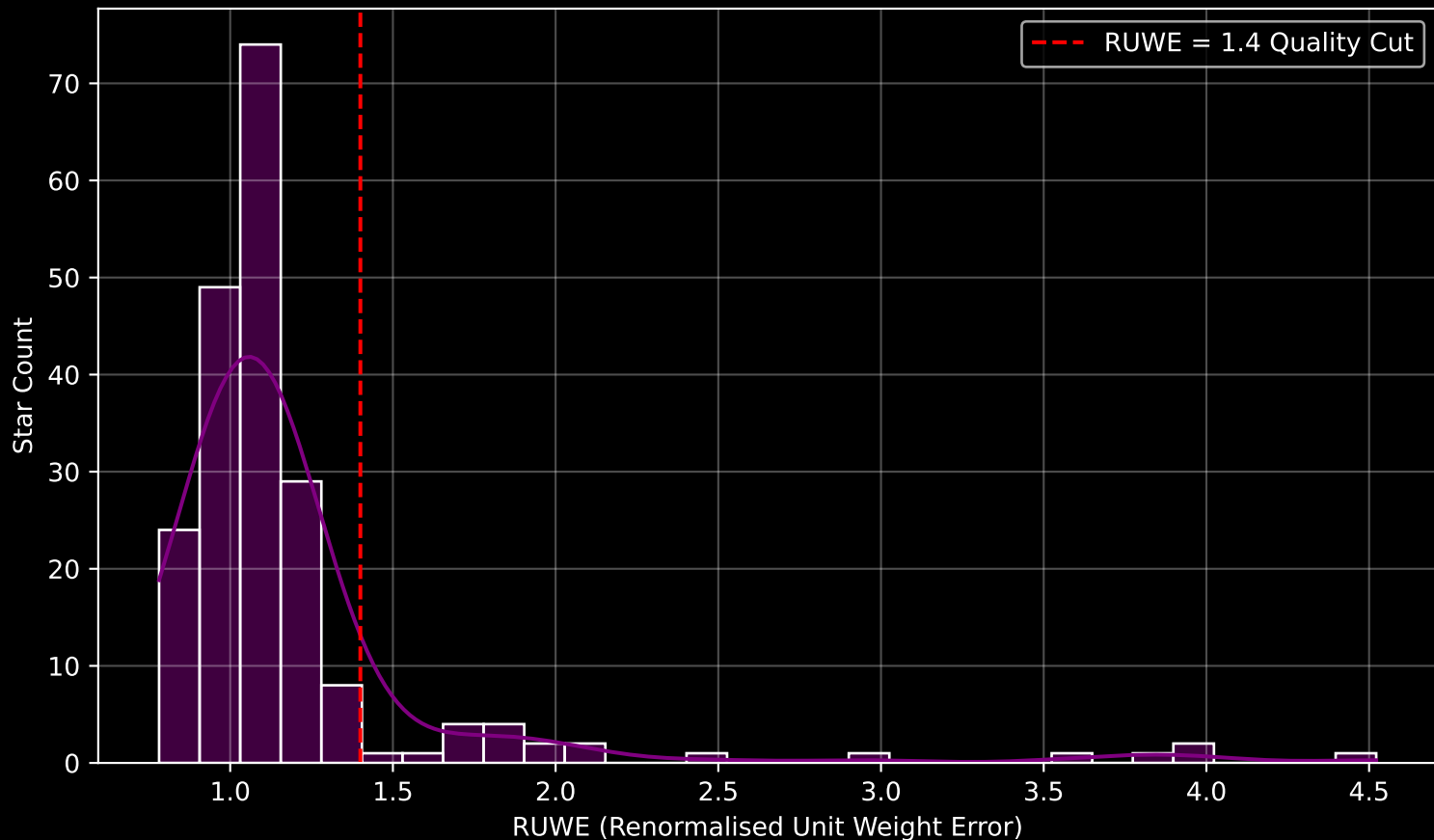
GALAH DR4 Field [7185] RUWE Distribution (n= 205)
