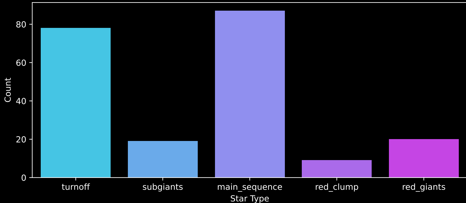
GALAH DR4 Field: [7185] Count plot of Star Type
